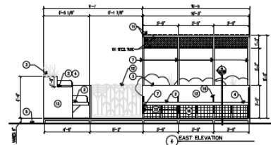
4 EAST ELEVATION
