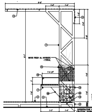
7 CROSS SECTION
