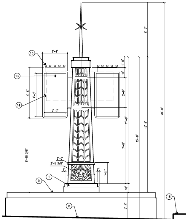
1 SPIRE ELEVATION
