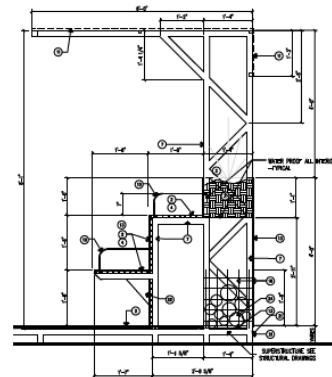
7 SECTION 02
