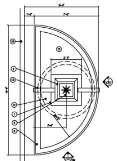
4 SPIRE FLOOR PLAN WEST
