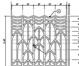
4 CAST ALUMINUM FENCE
