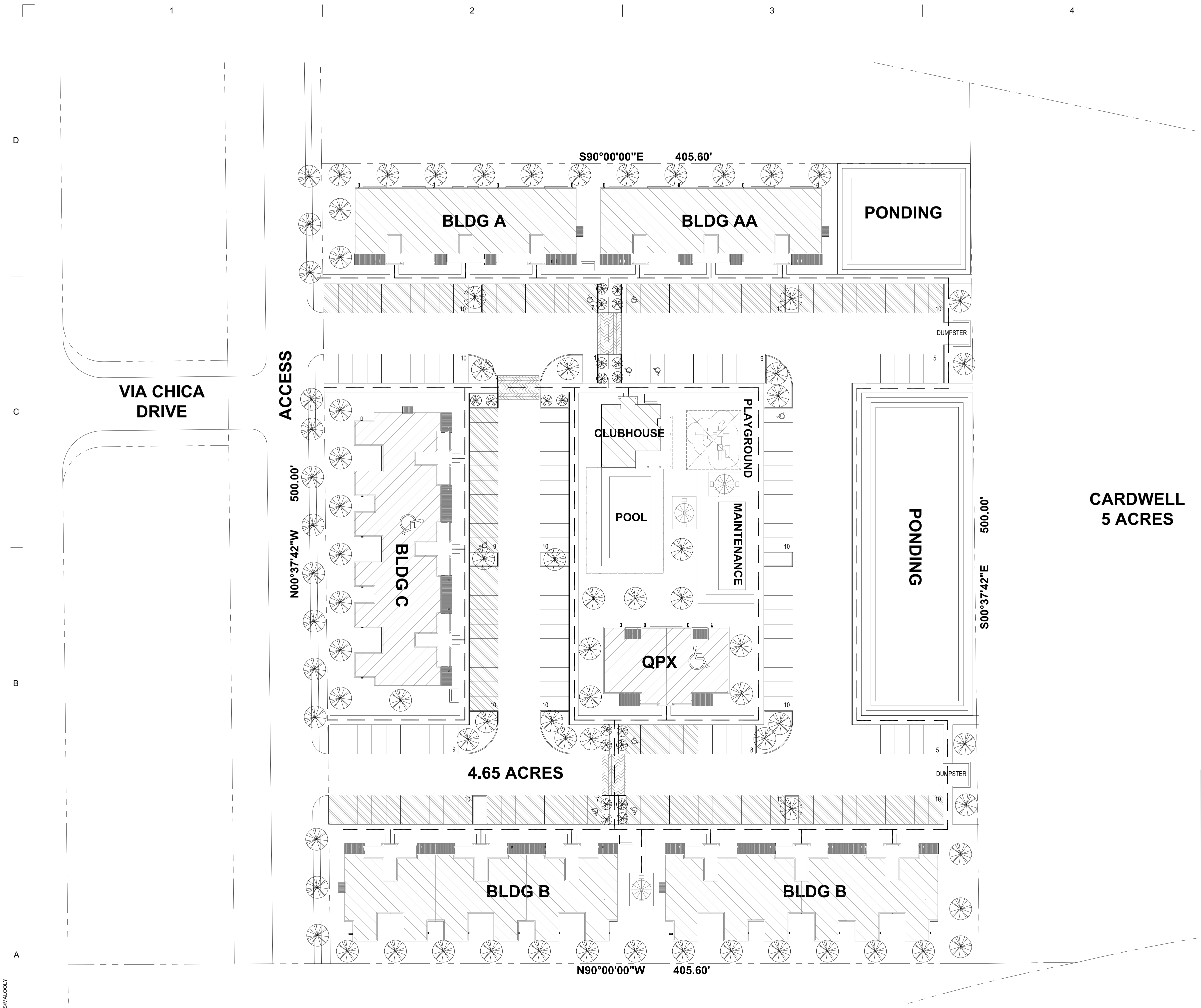
1 SITE PLAN 1" = 30'-0"
