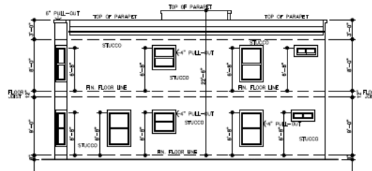
11. REAR ELEVATION
