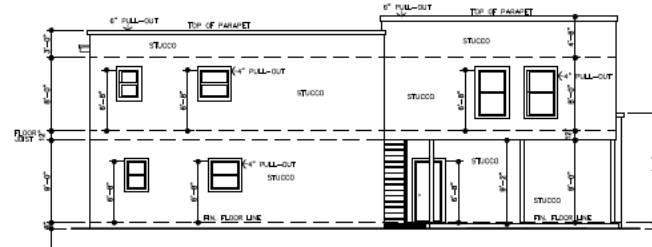
12. LEFT ELEVATION
