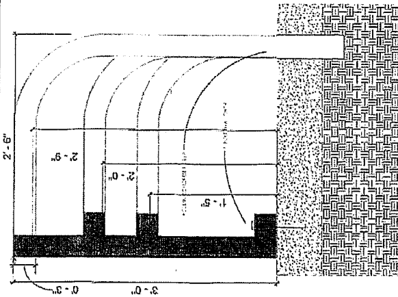
SIDE VIEW DETAIL OF BIKE RACK
