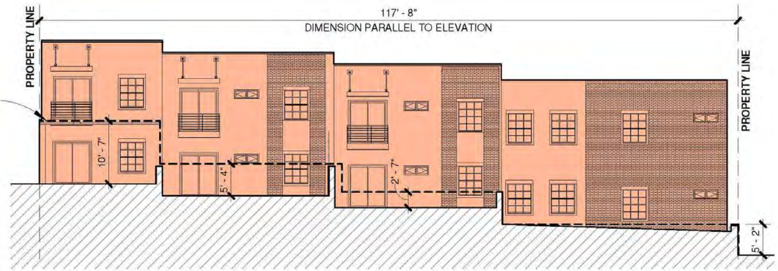
4 WEST ELEVATION 1" = 20'-0"
