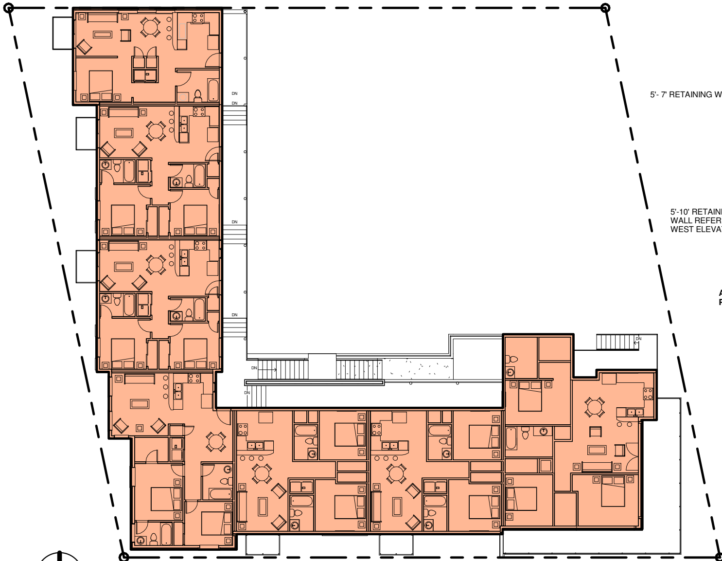
2 SECOND FLOOR PLAN 1" = 20'-0"
