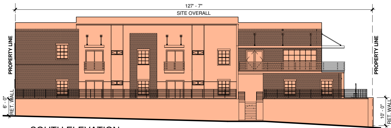
3 SOUTH ELEVATION 1" = 20'-0"
