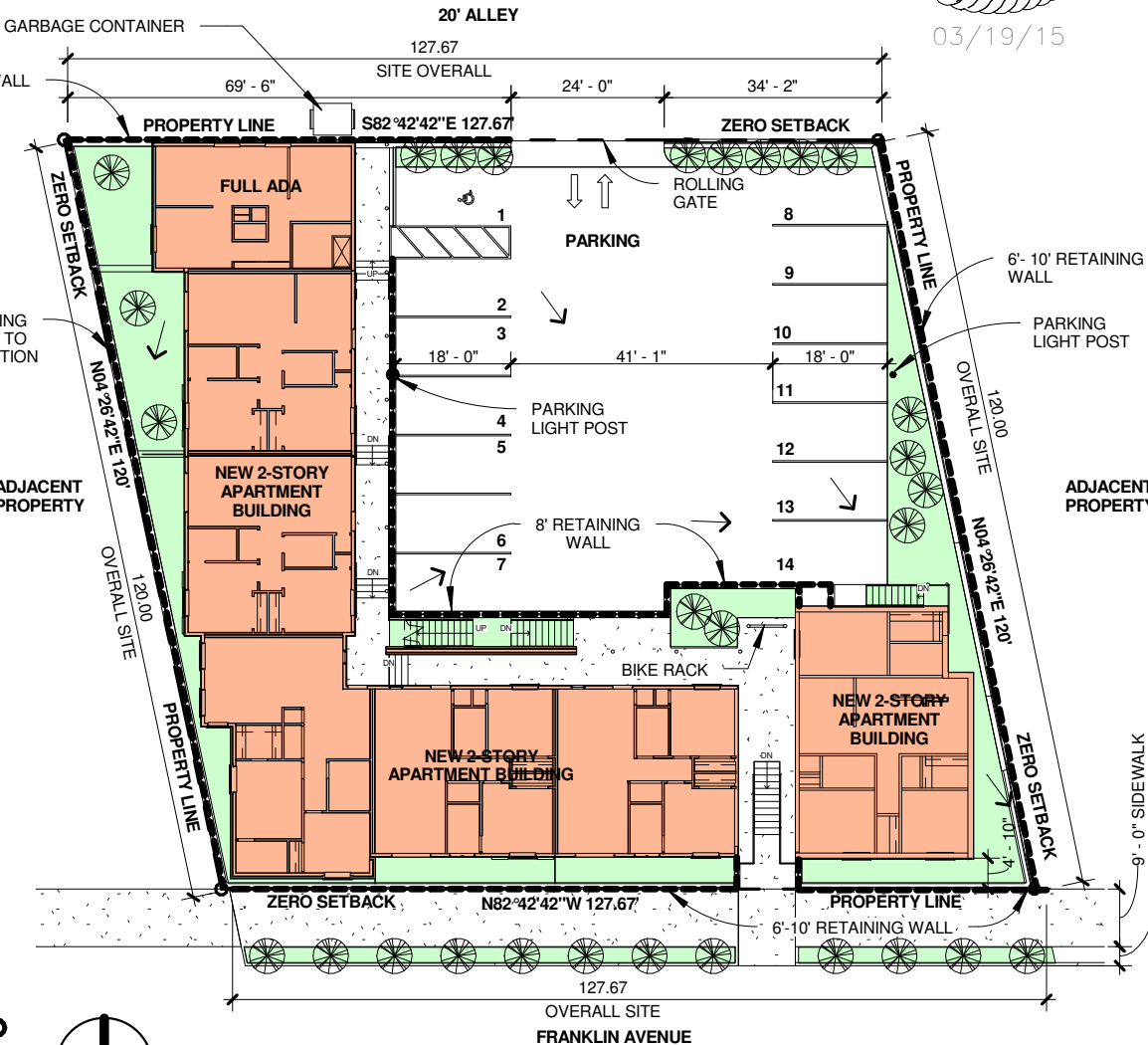
1 SITE PLAN 1" = 30'-0"
