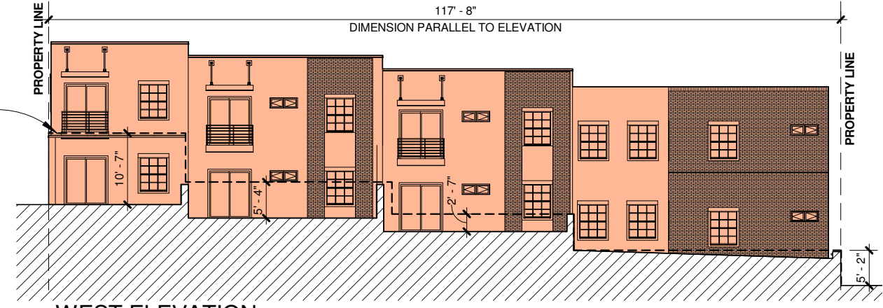
4 WEST ELEVATION 1" = 20'-0"
