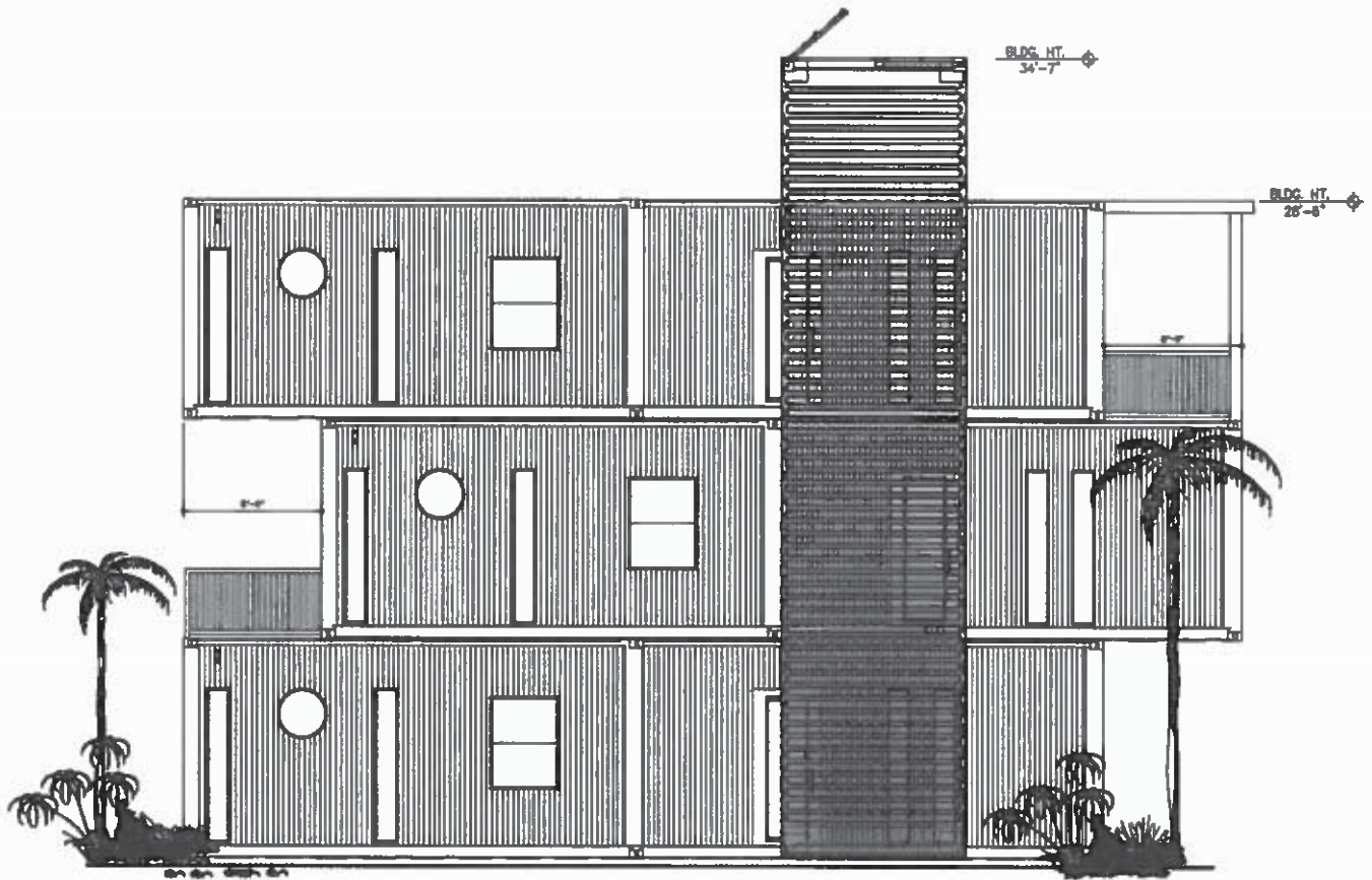
FRONT ELEVATION TRIPLEX
