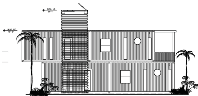
FRONT ELEVATION DUPLEX
