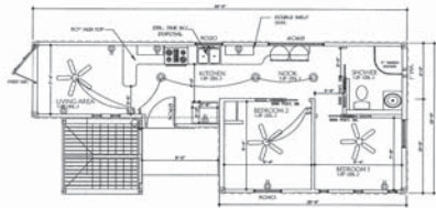
1ST FLOOR PLAN APARTMENT 1 Type "A" Unit-Fully Accessible
