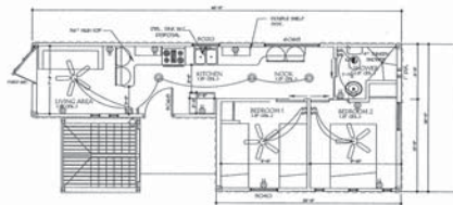
2ND FLOOR PLAN 3RD FLOOR PLAN APARTMENT 2&3
