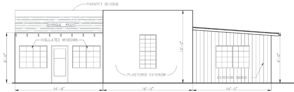
RESIDENCE ELEVATION SCALE: 1/4"=1'-0"
