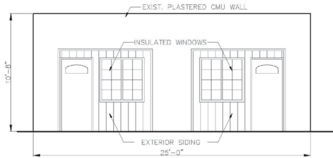
GARAGE CONVERSION ELEV. SCALE: 1/4"=1'-0"
