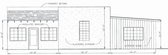
RESIDENCE ELEVATION SCALE: 1/8"=1'-0"
