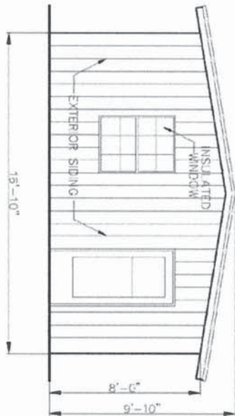
APARTMENT ELEVATION SCALE: 1/4"=1'-0"
