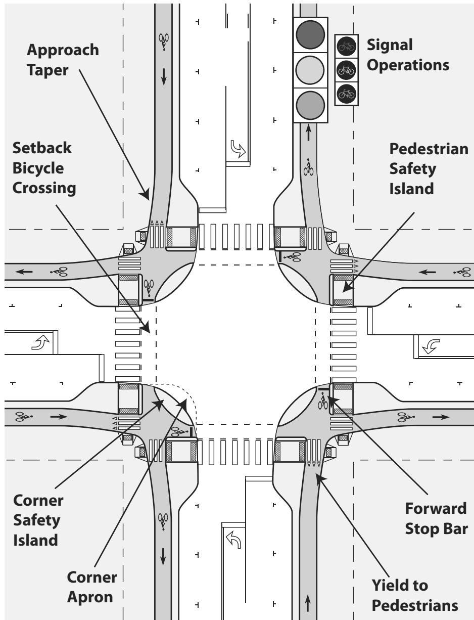
Figure C27. Visual illustration of key protected intersection features
