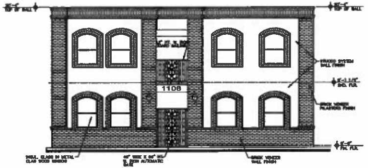
NORTH ELEVATION (FRONT)
